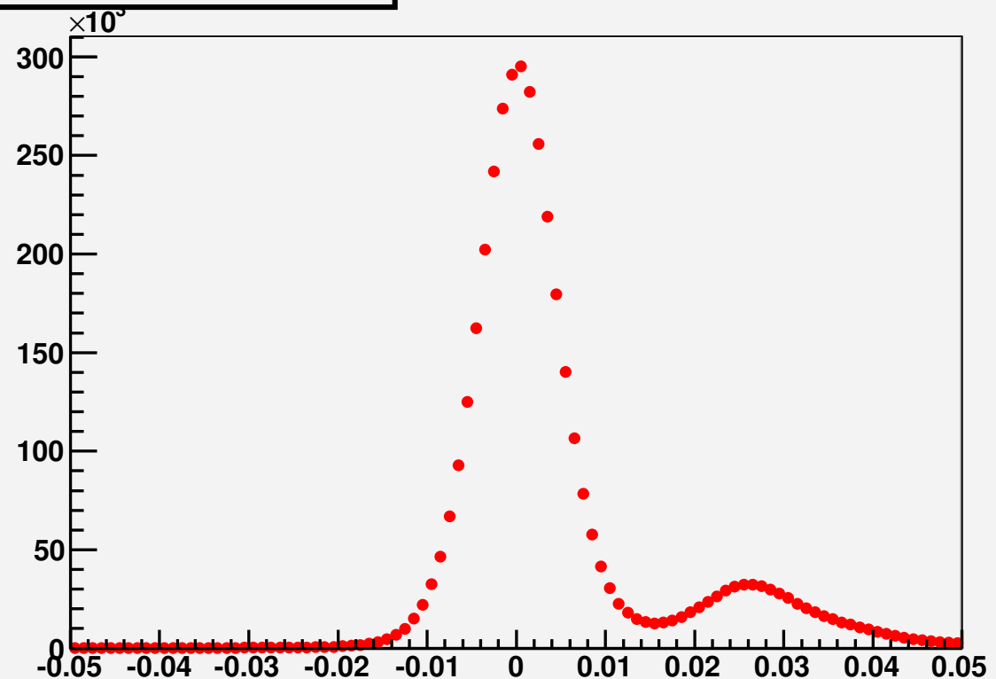
Missing mass distribution, K_{\mu2}
